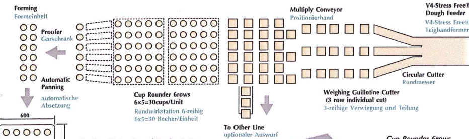
Cup Rounder 6rows Cup Rounder (Rundwirker) 6-reihig
